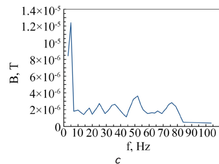
Fig. 1. Shielding of the magnetic field of an alternating-current electric machine by the textile material containing ferromagnetic nanostructures:
