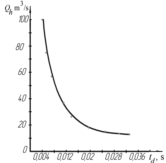
Fig. 4. Graph of the time delay operation hydraulic blanking dynamic fluctuations of supply of hydraulic fluid
